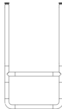
INFINITO CEILING BAR H 910 L 500 mm
